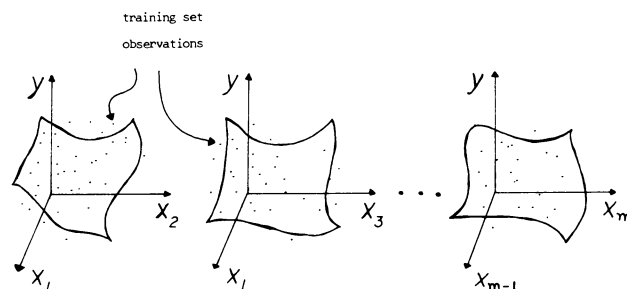
Figure 2. Construction of the New Variables
