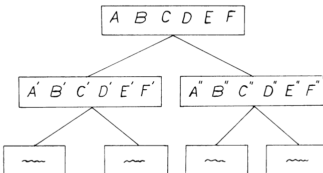
Figure 6. Tree of Polynomials Describing the Ivakhnenko Polynomial
